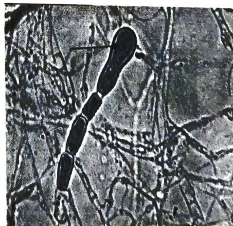
FIGURE: CHLAMYDOSPORES
