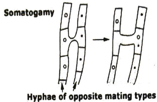
FIGURE: SOMATOGAMY
