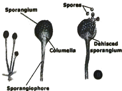
FIGURE: CONIDIOPHORES
