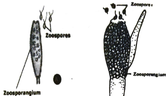
FIGURE: ZOOSPORES
