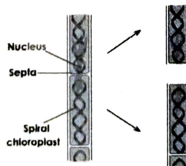
FIGURE: FRAGMENTATION
