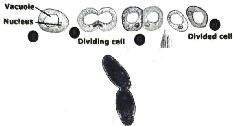
FIGURE: FISSION
