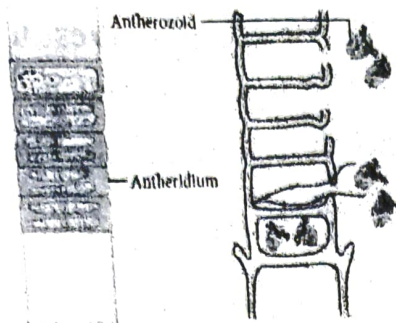
Antherozoid formation and liberation
