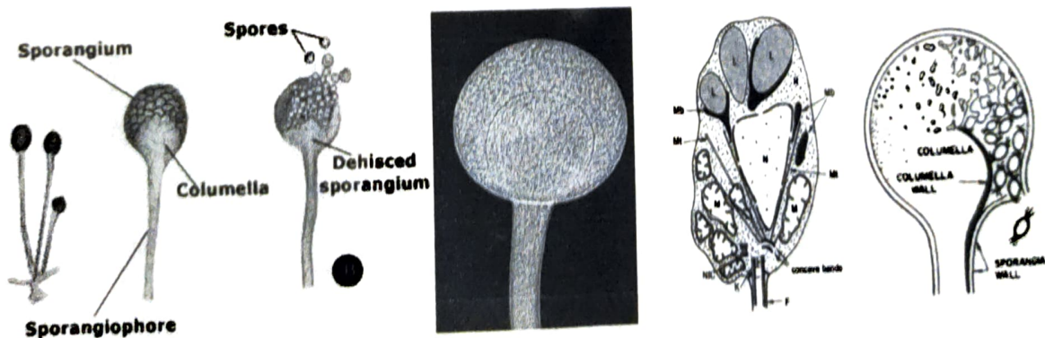
FIGURE: ALL ARE SPORANGIOSPORES
