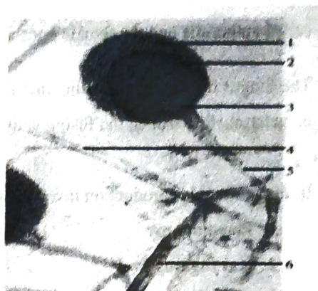
Figure 5.4 A whole mount of the bread mold Rhizopus . 1. Sporangium 2. Spores 3. Columella 4. Rhizoid 5. Sporangiophore 6. Stolon (hyphae)
