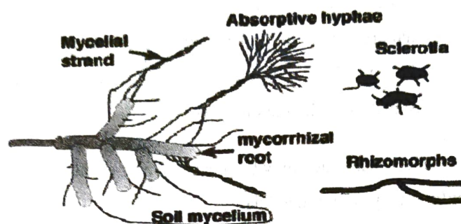
FIGURE: RHIZORNORPHS
