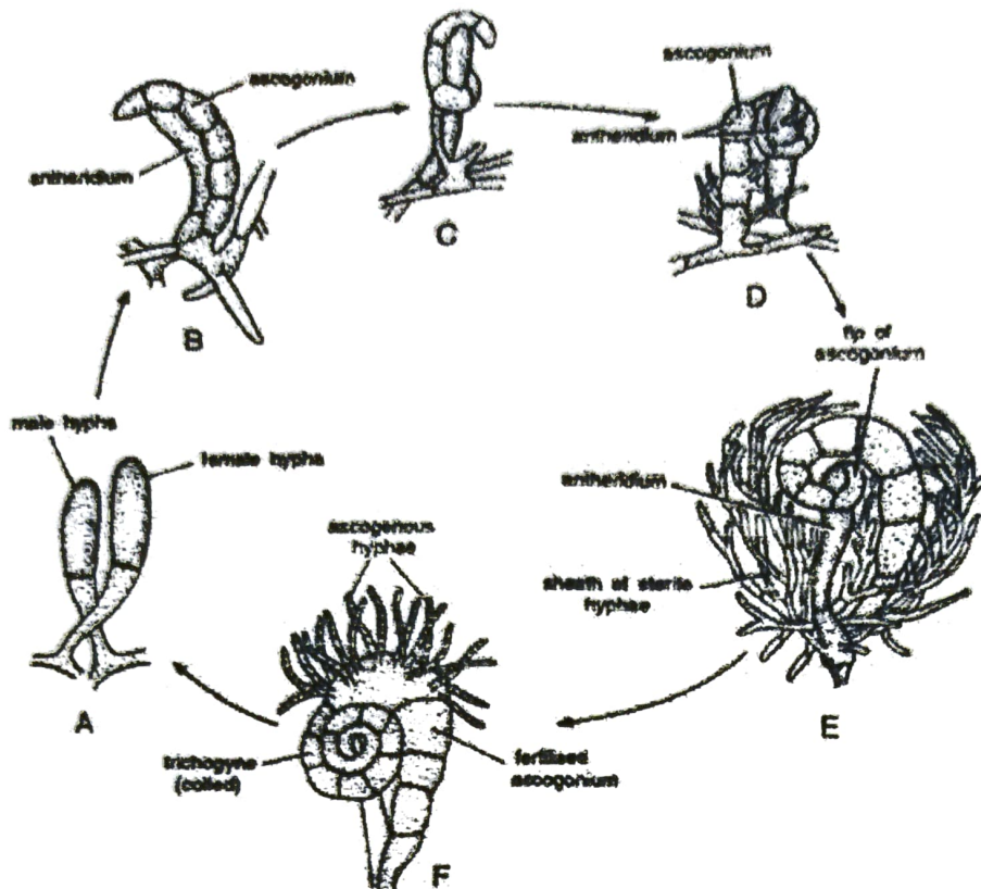
Fig. 3. Ascobolus . Sexual reproduction
