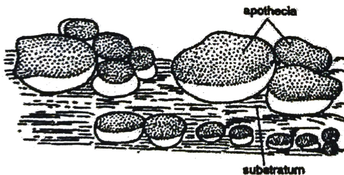
Fig. 1. Ascobolus : Aerial apothecia.
