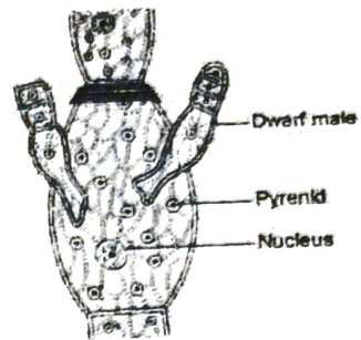
Dwarf male on oogonial wall
