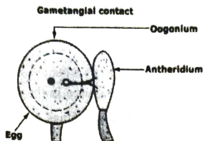
FIGURE: GAMETANGIAL CONTACT
