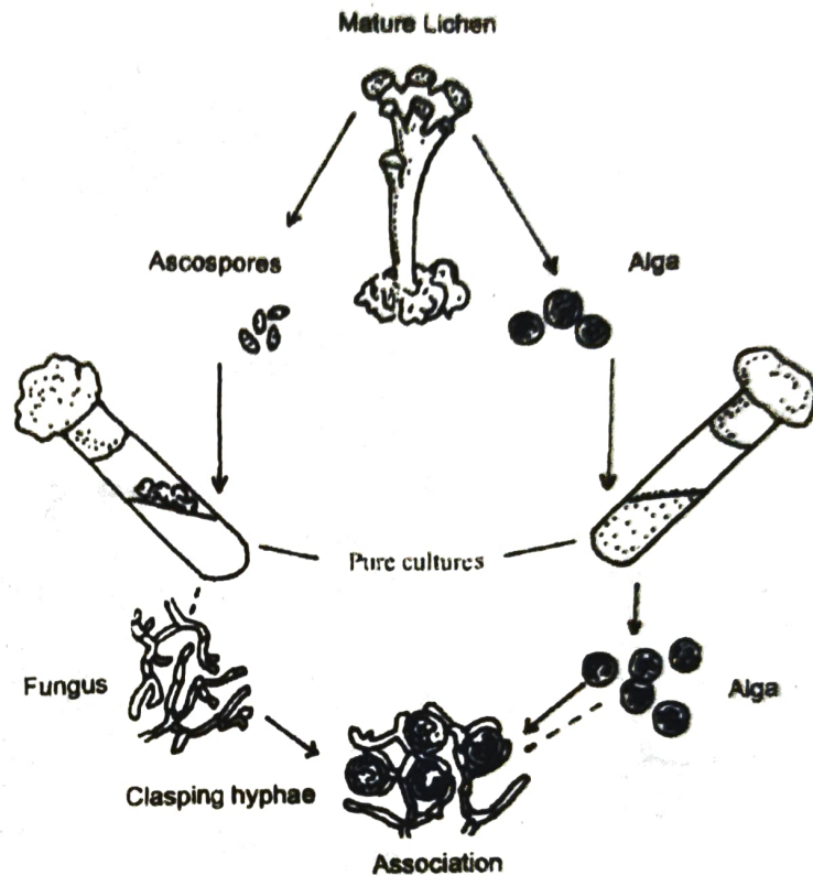
Fig. 12.1: Diagrammatic representation showing separation and culture of lichen components and the reconstruction of lichen from them.
