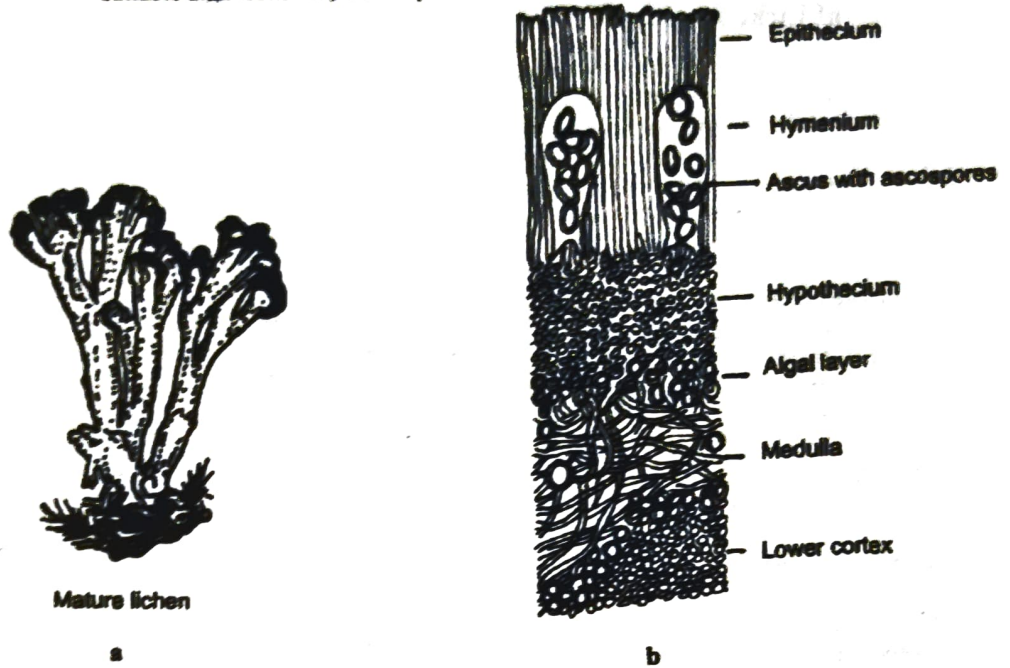
Fig. 12.5: Reproductive structures in lichens: a) apothecia, b) cross section of a typical apothecium.
