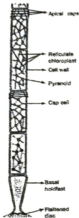
a) A part of filament
