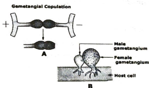
FIGURE: GAMETANGIAL COPULATION
