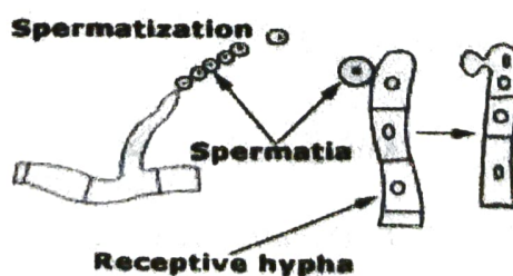
FIGURE: SPERMATIZATION
