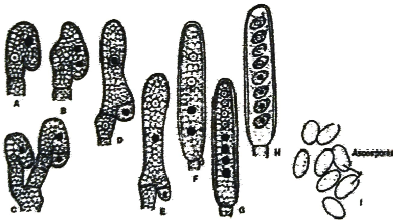
Fig. 4. Ascoascus , formation of Ascospores
