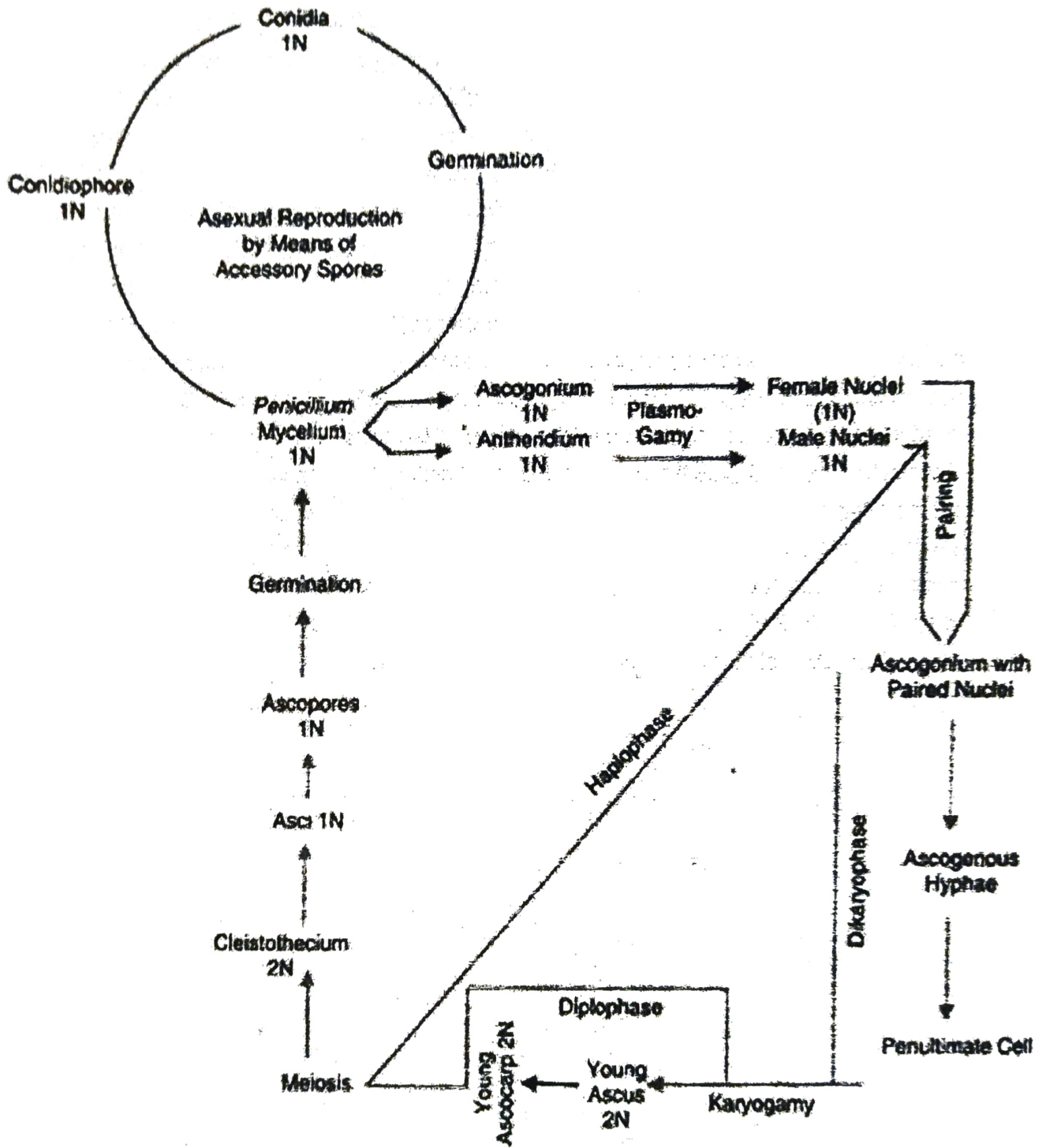
Fig. 10.20. Graphic representation of the life cycle of Penicillium sp.
