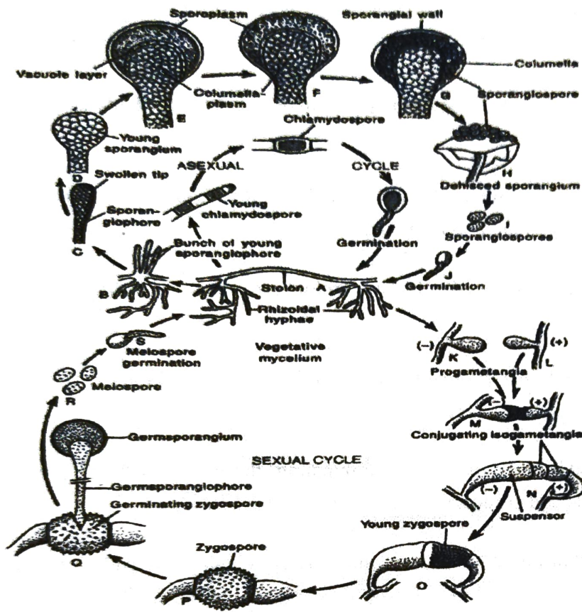
Fig. 4.26 : Life cycle of Rhizopus stolonifer
